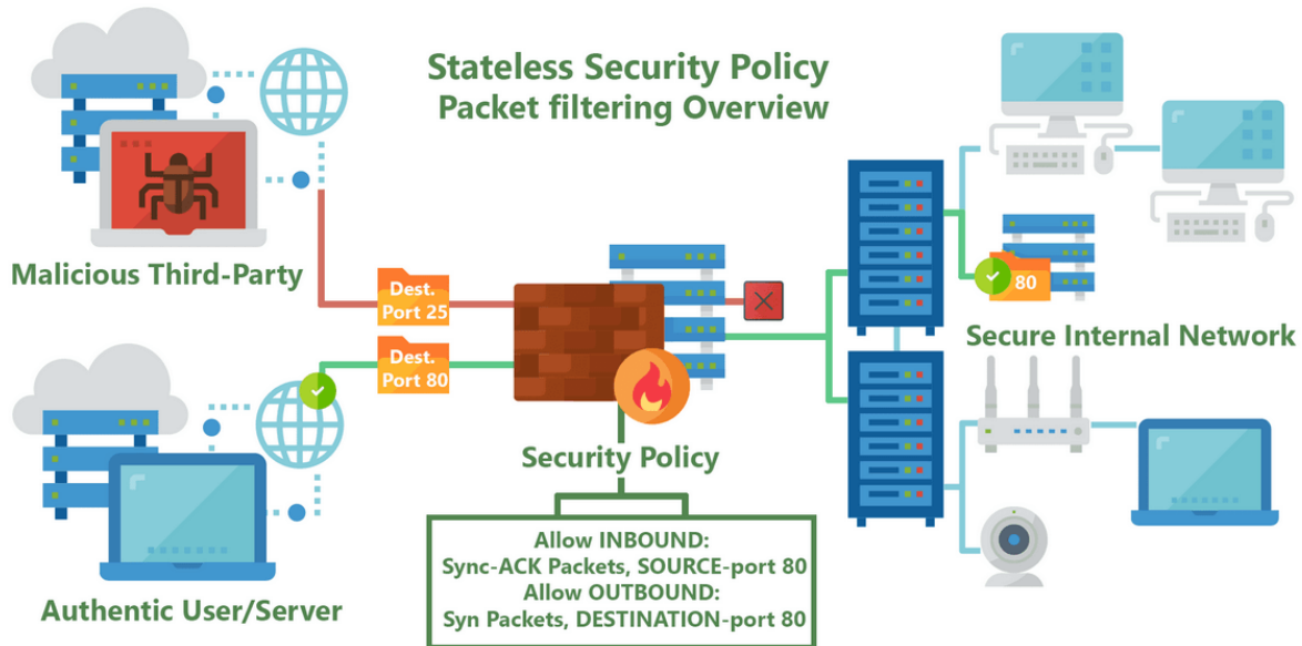
Packet Filtering Firewall (layer-4)
